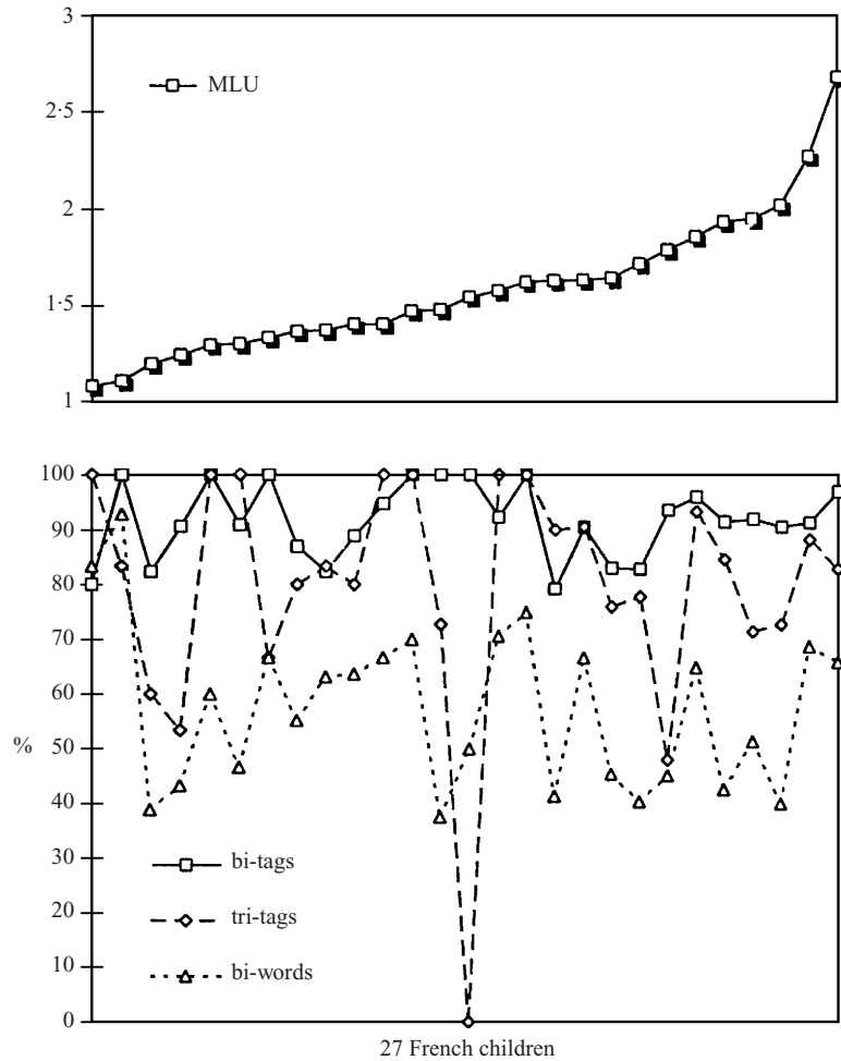
Fig. 1. MLU for each of the 27 children and coincidence percentages of bi-tags, tri-tags and bi-words production between each of the 27 children and the adults. (Note: 1. Points in the same vertical line correspond to one child, be they on the MLU, or the bi-tags, tri-tags or bi-words plot graphs. The two figures are separated because the scales are different. 2. MLU value is given in words per utterance.)
